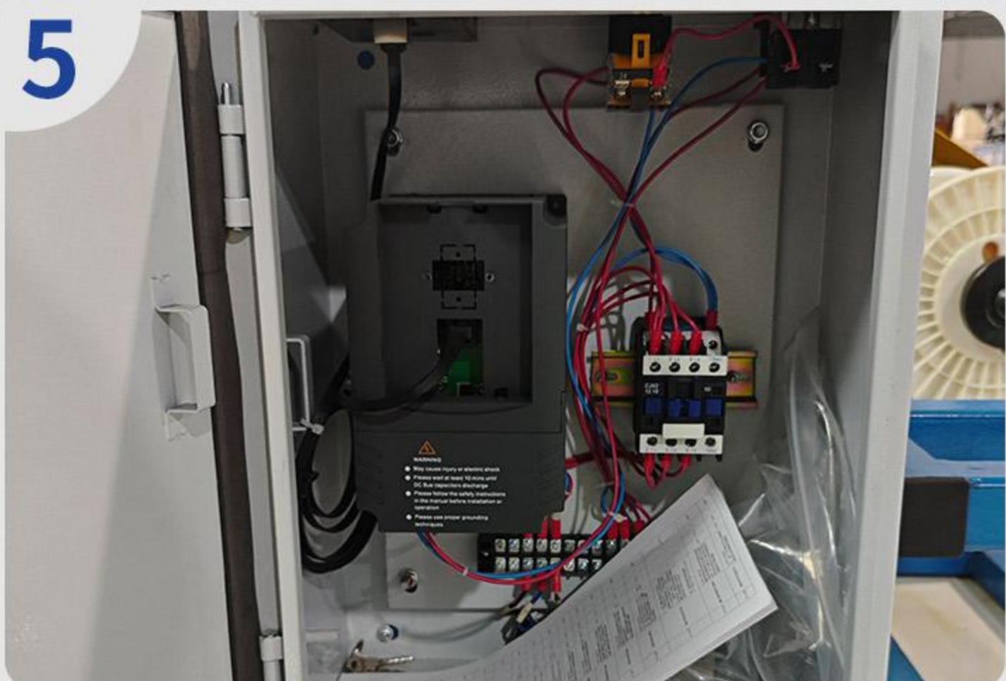
Electrical Enclosure
